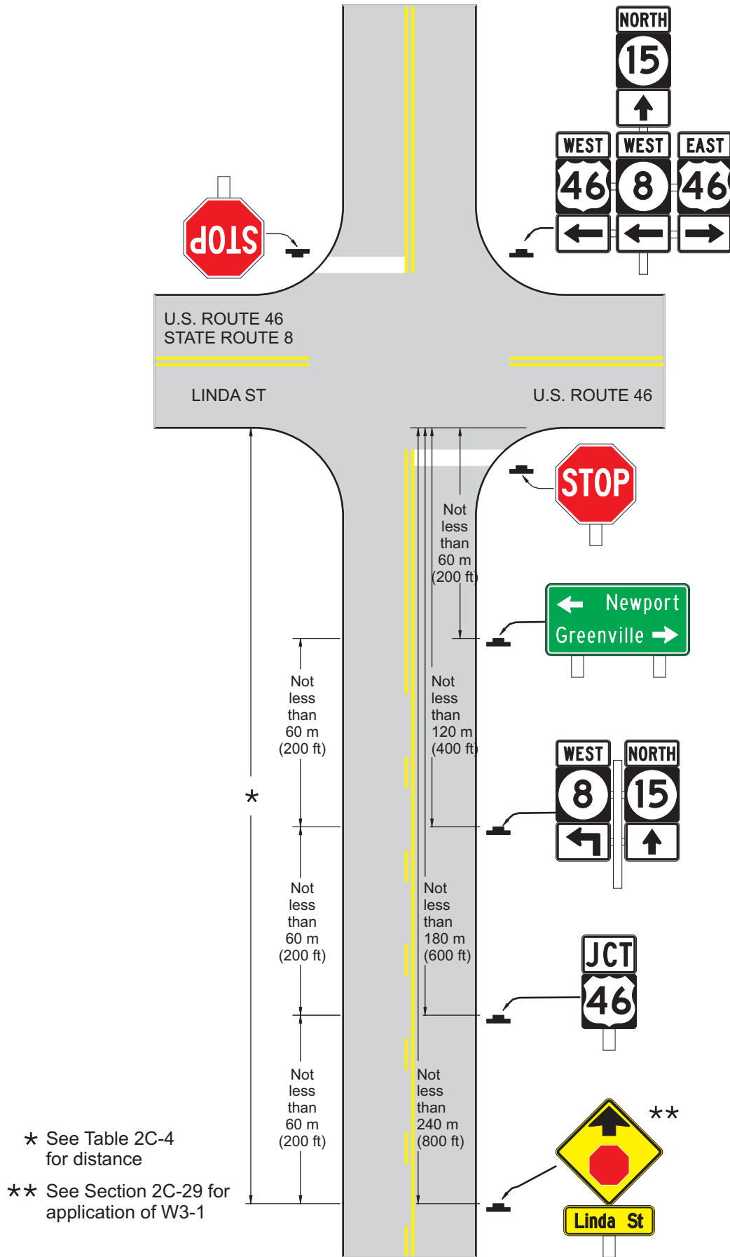
Figure 2A.04. Illustration of Guidance & Warning signs (sheet 2 of 3)
